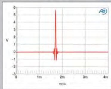
Fig.1 Gryphon Ethos, Filter 2, impulse response (one sample at OdBFS, 4ms time window).
