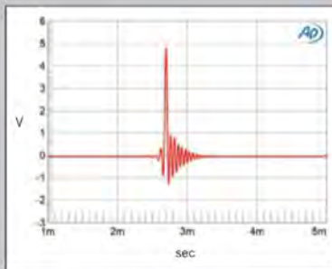
Fig.3 Gryphon Ethos, Filter 4, impulse response (one sample at OdBFS, 4ms time window).
