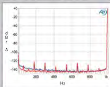
Fig.9 Gryphon Ethos, spectrum with noise and spurs of a dithered 1kHz tone at 0dBFS (left channel blue, right red) (20dB/vertical div.).
