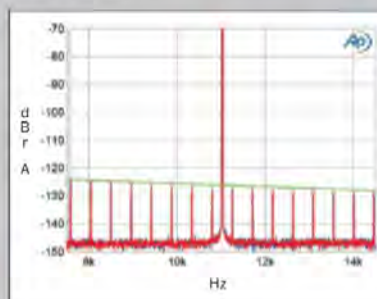
Fig.15 Gryphon Ethos, high-resolution jitter spectrum of analog output signal, 11.025kHz at -6dBFS, sampled at 44.1kHz with LSB toggled at 229Hz; CD data (left channel blue, right red). Center frequency of trace, 11.025kHz; frequency range, \pm 3.5 kHz.
