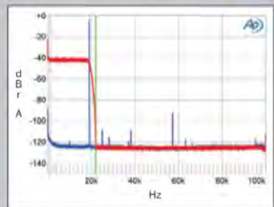
Fig.6 Gryphon Ethos, Filter 4, wideband spectrum of white noise at -4dBFS (left channel red, right magenta) and 19.1kHz tone at 0dBFS (left blue, right cyan), with CD data (20dB/vertical div.).
