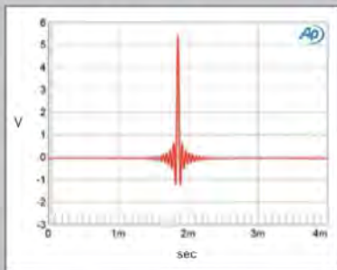
Fig.2 Gryphon Ethos, Filter 3, impulse response (one sample at OdBFS, 4ms time window).
